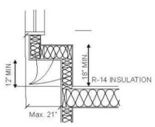
Detail "B" Typical Bay Window
