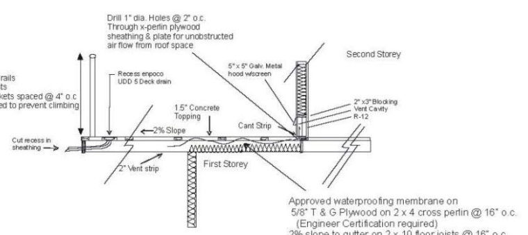
Detail "D" - Typical deck over living area detail
